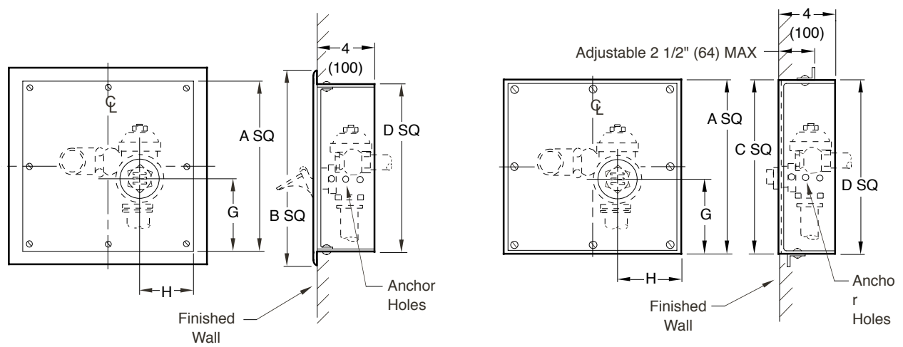
Fig. 4740 FACE-OF-WALL BOX
