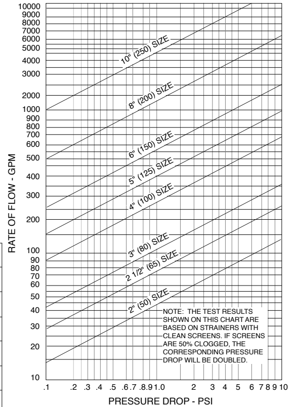
PRESSURE DROP THROUGH FIG. 8790 AND FIG. 8795 AT VARIABLE FLOW RATES
