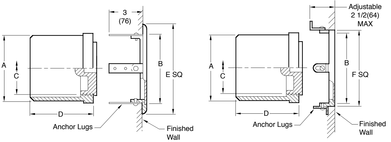
FIG. 4434C . . . . FACE-OF-WALL COVER
