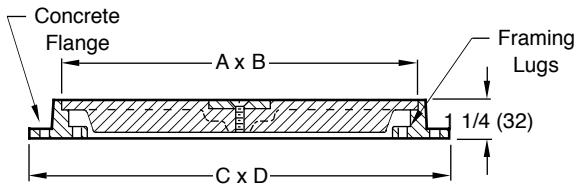
Fig. 4910 . . . . . SECURED COVER
