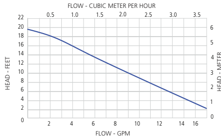
Single Speed AM8 & AM10 Single Speed
