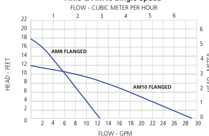
Single Speed AM8 & AM10 Single Speed
