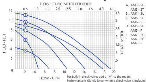
Single Speed Curves, AM1 to AM7 S-Stainless, U-Union, T-Threaded, F-Flanged
