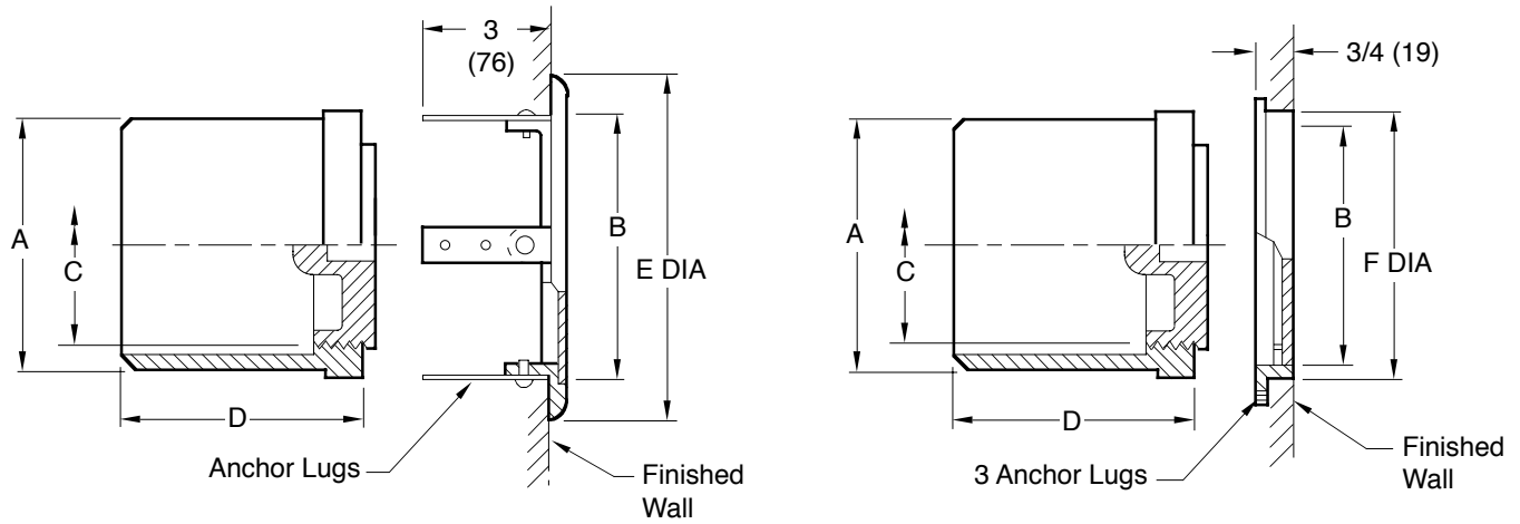
FIG. 4436C . . . . FACE-OF-WALL COVER
